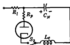
FIG. 11-20.—Schematic diagram of the potential-reversing circuit.
